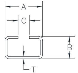
C Channel
