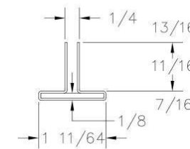
Slotted Standard
